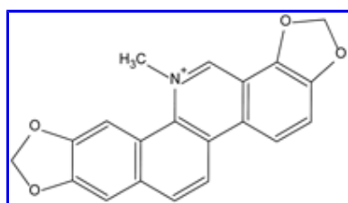
Fig. 1. Structure of sanguinarine.
